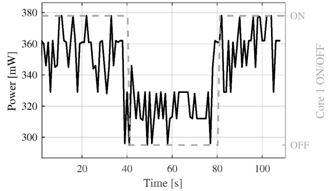
Figure 6. Experimental measurement obtained by applying core suspension .
